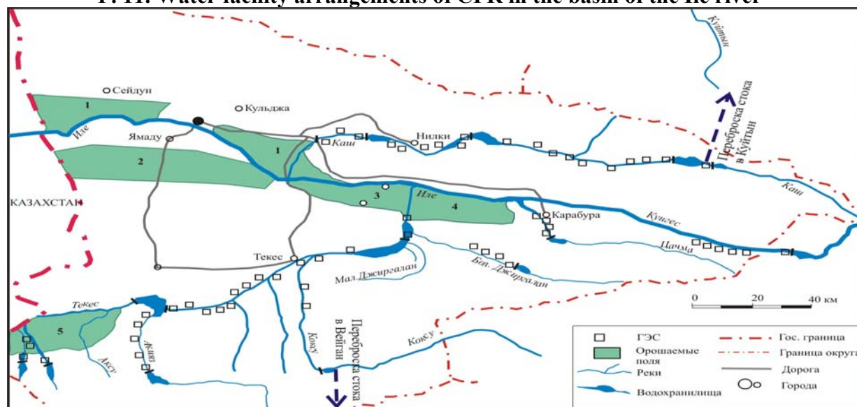
P. 11. Water facility arrangements of CPR in the basin of the Ile river
